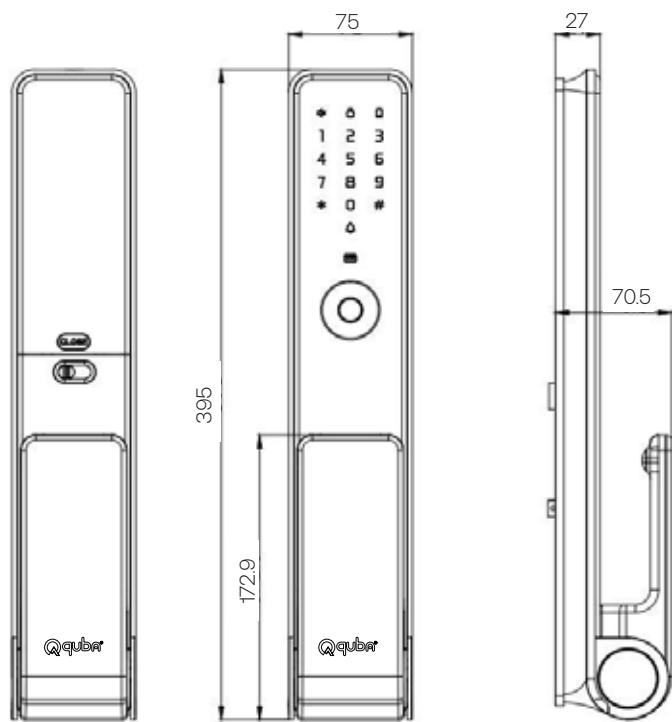
QUANTRA: Push & Pull 5-Way Access Digital Lock
